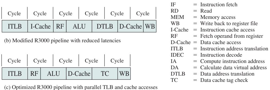
Figure 15.10 Enhancing the R3000 Pipeline
